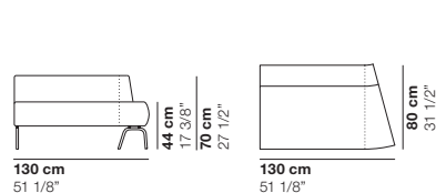
cod. 1197 / right open element 130 15° R110
