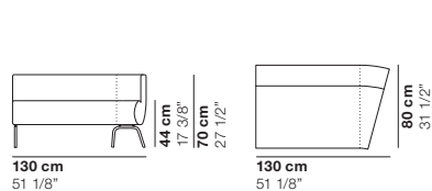
cod. 1195 / right closed element 130 15° R110
