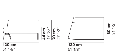
cod. 1196 / left open element 130 15° R110
