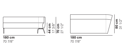
cod. 1199 / right closed element 180 15° R110
