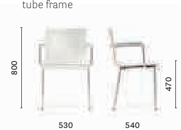
2444 * Armchair, plywood shell upholstered front side, steel tube frame
