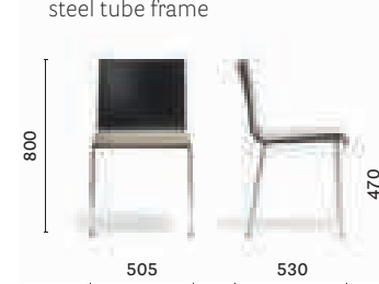
2413/A * Side chair, plywood shell, upholstered seat, steel tube frame
