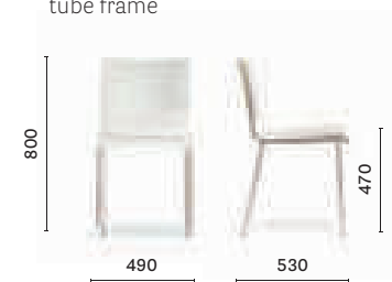
2441 * Side chair, plywood shell upholstered front side, steel tube frame
