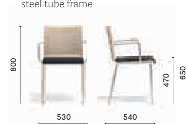
2414/A * Armchair, plywood shell, upholstered seat, steel tube frame
